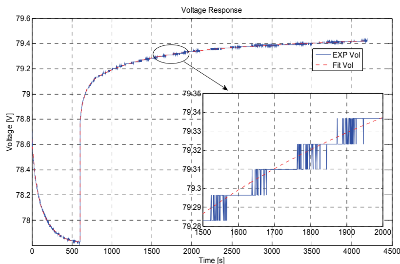
Fig. 4. Experimental voltage and fitted voltage.
