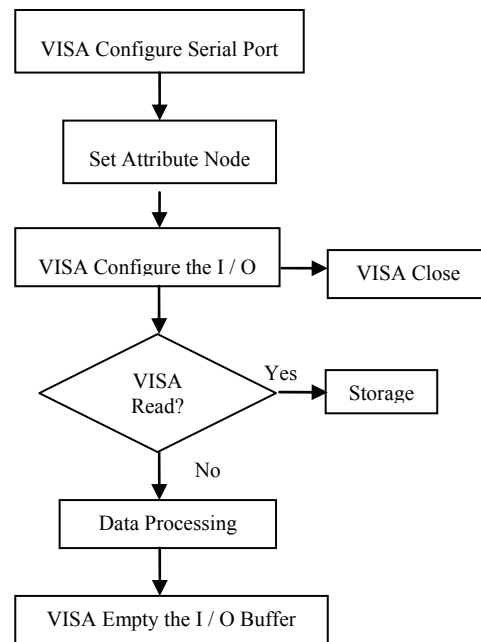
Fig. 3. VISA Read the Serial Flow Chart.
