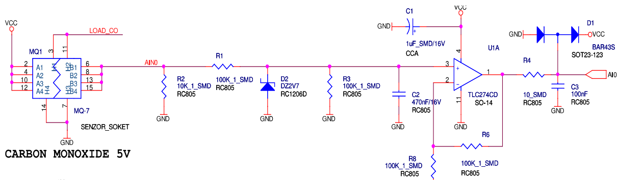
Fig. 3. Circuit Diagram for CO Sensor Integration.
