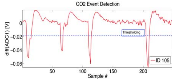
Fig. 5. Event Detection based on Acquired Data.
