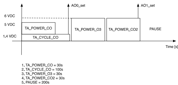
Fig. 6. Periodic Sampling of the Gas Sensors.
