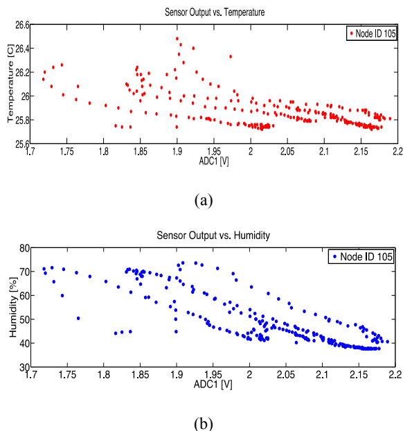
Fig. 7. CO 2 Sensor Output vs. Ambient (a) Temperature (b) Humidity.
