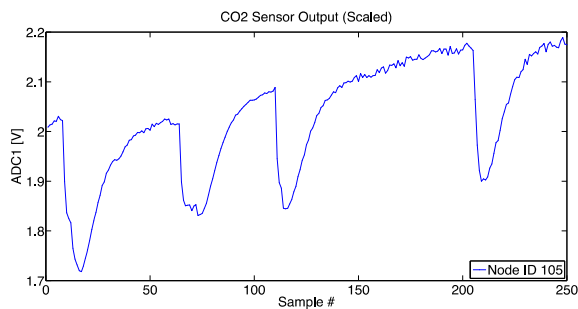
Fig. 4. Carbon Dioxide Sensor Output.
