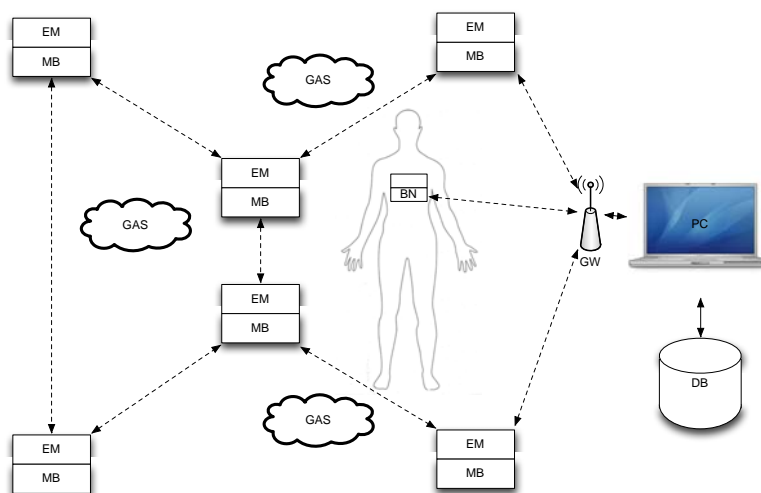
Fig. 1. Wireless Gas Sensor Network (WGSN).
