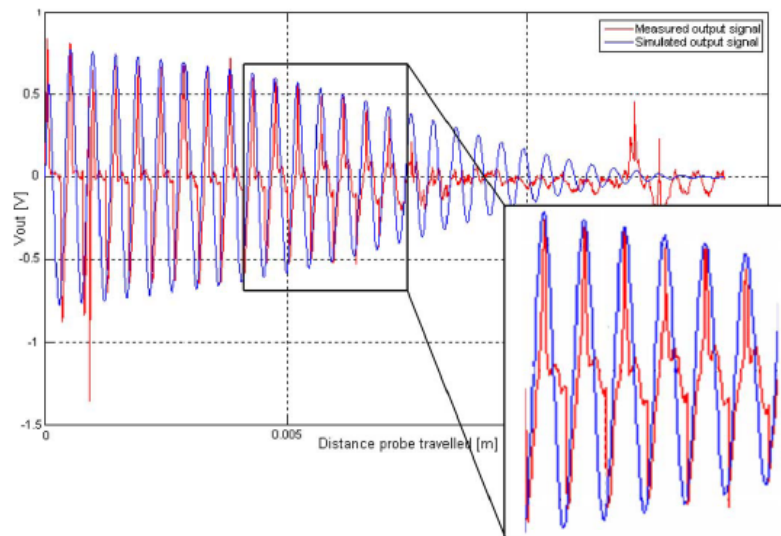
Fig. 10. Sensor output signal while the probe is moved through the window in the tube under the cantilever target.
