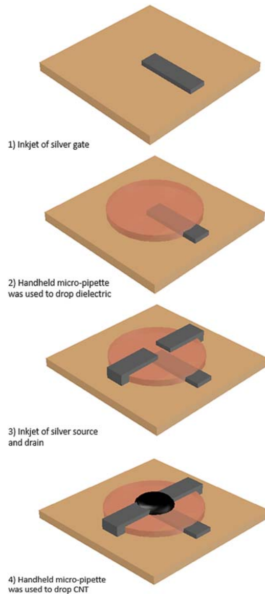
Fig. 3. 3D illustration of CNT TFT fabrication process.
