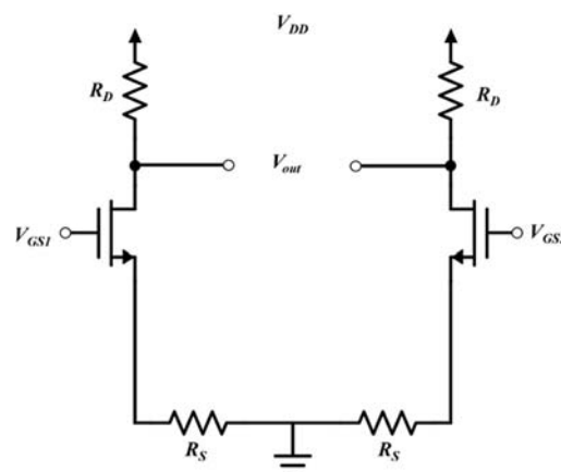
Fig. 2. Schematic of a MOS-based differential amplifier.
