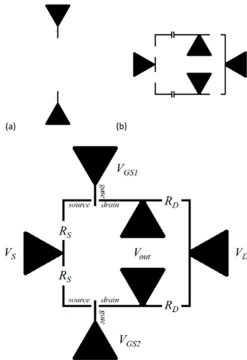
Fig. 4. Bitmap image files of printed patterns. (a) gate, (b) source and drain (adjacent T shapes) and circuit.
