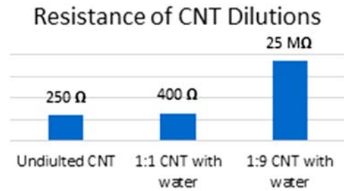
Fig. 5. Resistance of CNT Dilutions.
