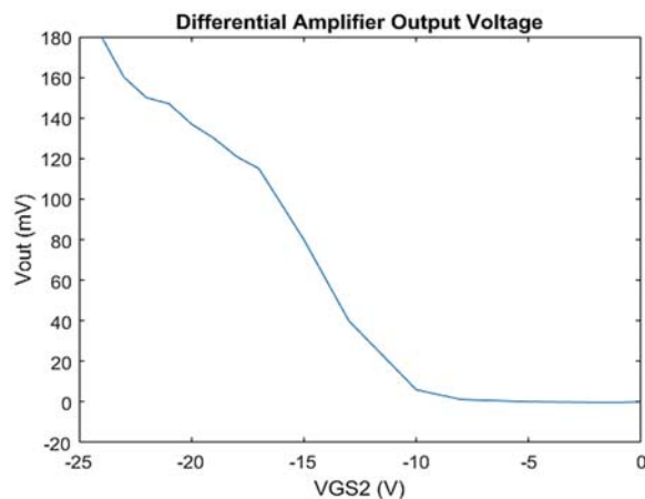
Fig. 8. Chart of output voltage of differential amplifier.
