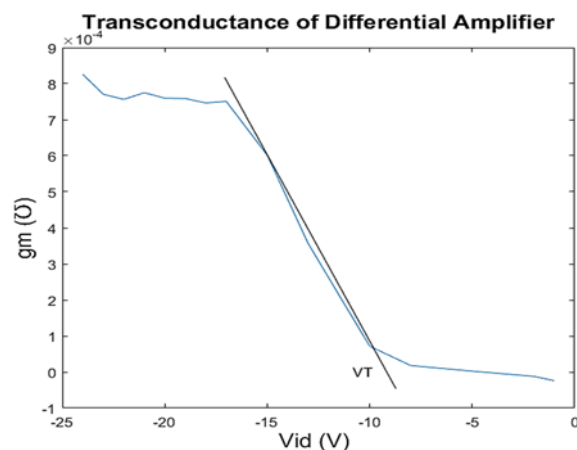
Fig. 9. Transconductance of differential amplifier.
