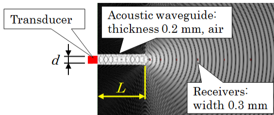
Fig. 2. Model for length of acoustic waveguide [15].
