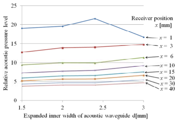
Fig. 7. Acoustic pressure characteristics due to expanding inner width of acoustic waveguide.
