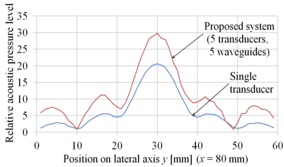
(a) Comparison of peak acoustic pressure.
