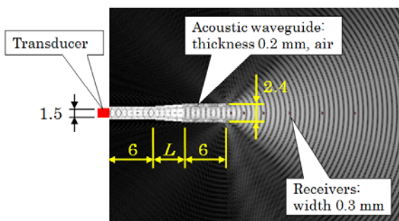
Fig. 8. Model for expansion length of acoustic waveguide.
