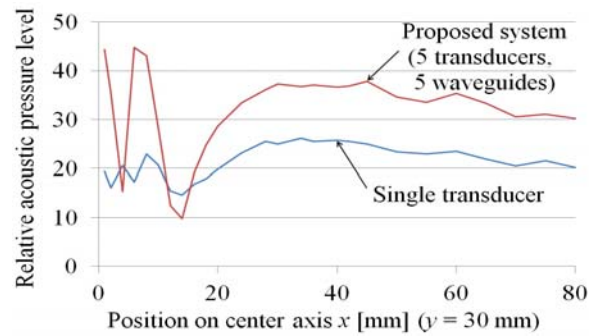
Fig. 19. Comparison of the center acoustic pressure [15].
