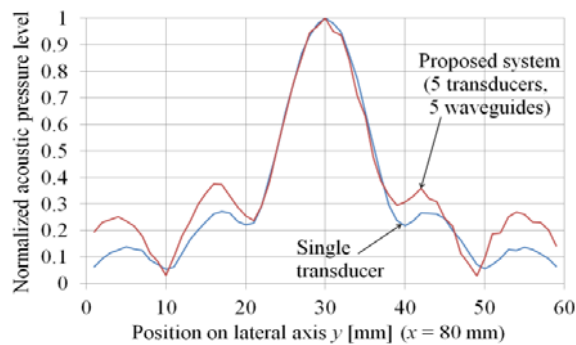
(b) Comparison of beam width of normalized acoustic pressure.
