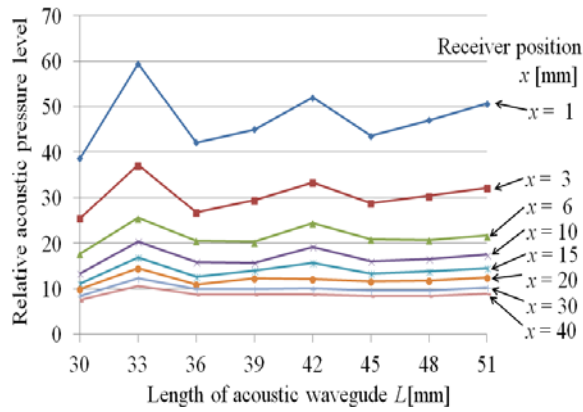
Fig. 11. Acoustic pressure characteristics due to focusing with acoustic waveguide [15].
