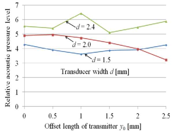
Fig. 5. Acoustic pressure characteristics due to bending of acoustic waveguide ( x = 30 mm) [15].
