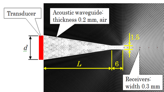
Fig. 10. Model for focusing with acoustic waveguide [15].
