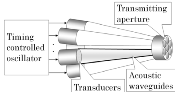
Fig. 1. Ultrasonic source system using multiple acoustic waveguides and piezoelectric transducers [15].
