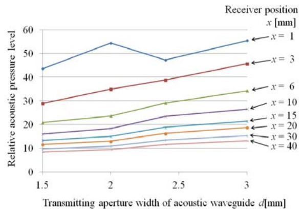
Fig. 15. Acoustic pressure characteristics due to transmitting aperture width of acoustic waveguide.
