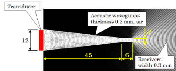
Fig. 14. Model for transmitting aperture width of acoustic waveguide.
