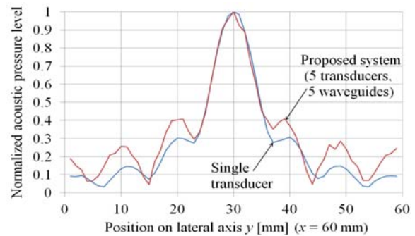
(b) Comparison of beam width of normalized acoustic pressure.
