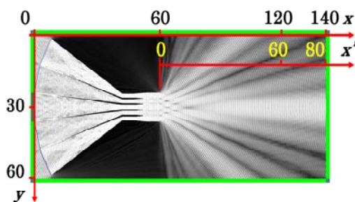
Fig. 18. Spatial distribution of displacement with the proposed system (absolute value) [15].
