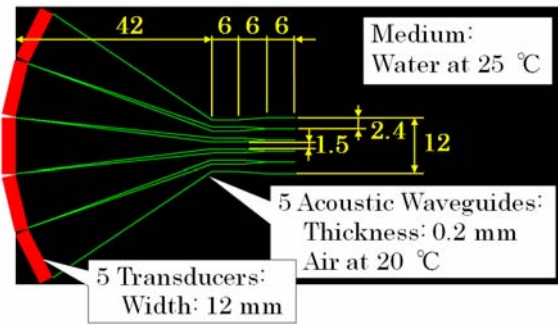
Fig. 16. Two-dimensional simulation model of the proposed system [15].
