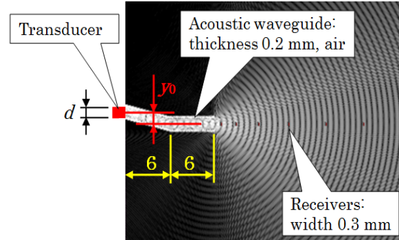
Fig. 4. Model for bending of acoustic waveguide [15].
