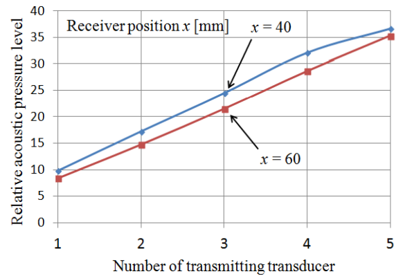
Fig. 22. The relationships between maximum acoustic pressure levels and number of transmitting transducers [15].
