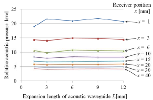
Fig. 9. Acoustic pressure characteristics due to expansion length of acoustic waveguide.
