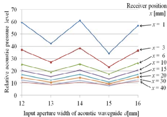
Fig. 13. Acoustic pressure characteristics due to expanding input aperture width of acoustic waveguide.
