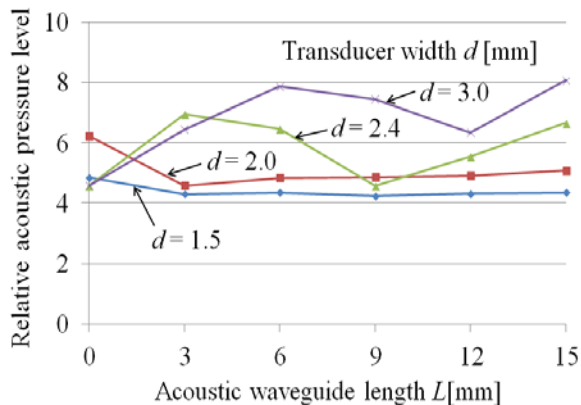
Fig. 3. Acoustic pressure characteristic due to length of acoustic waveguide ( x = 30 mm) [15].
