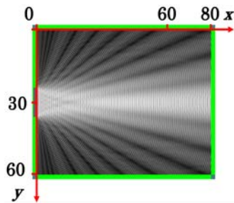
Fig. 17. Spatial distribution of displacement with a single transducer (absolute value) [15].
