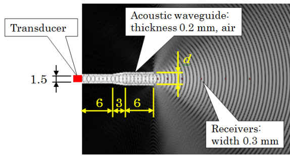
Fig. 6. Model for expanding inner width of acoustic waveguide.
