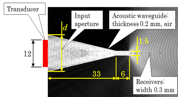
Fig. 12. Model for expanding input aperture width of acoustic waveguide.
