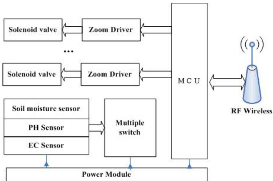
Fig. 2. Sensor nodes hardware control structure.
