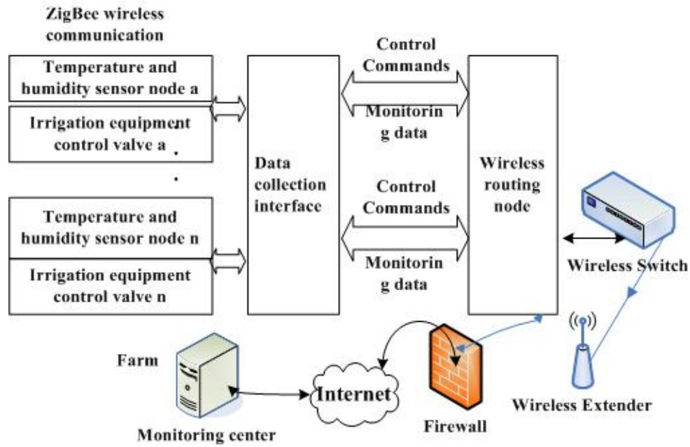
Fig. 1. Wireless sensor system structure.
