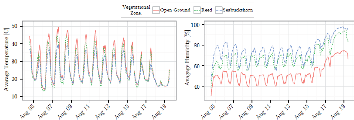
Fig. 10. Measured temperature and humidity as hourly average of all nodes within a vegetational zone.
