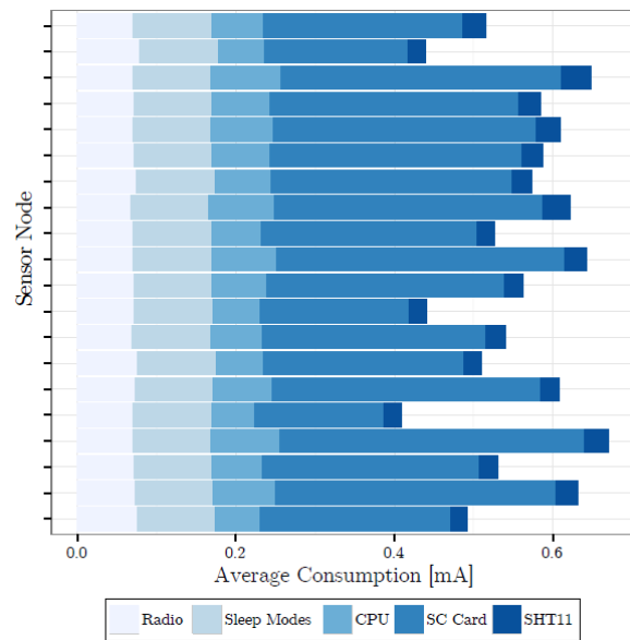
Fig. 12. Average accounted energy consumption of each sensor node.
