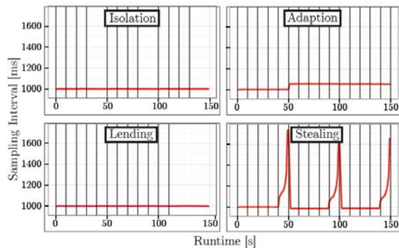
Fig. 4. Influence of different policies when more energy is needed than allocated.
