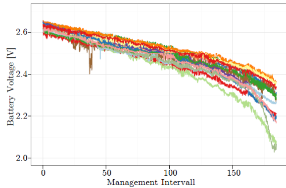
Fig. 13. Battery voltage of the nodes.
