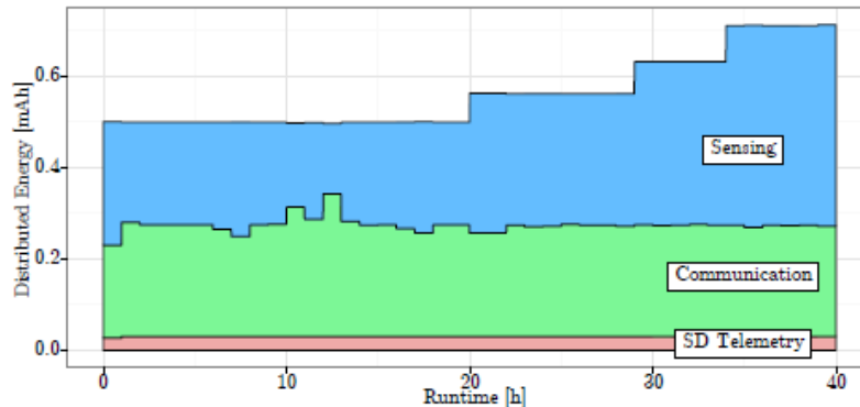
Fig. 7. Distributed energy to different application parts. Battery Manager increases available energy over time due to higher capacity than expected.
