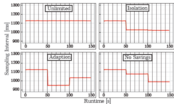
Fig. 5. Influences of the choice of policy if a task needs less energy than assumed.
