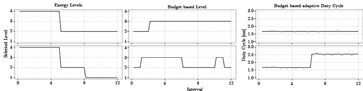
Fig. 6. Experimental comparison of management approaches. Energy Levels computes feasible level assignment based on available energy and level utility. Budget based Level assigns level based on available energy in budget. Budget based duty cycle is computed based on available energy and runtime cost. Lower half shows experiment where in interval 6 the available energy was reduced by 20 %.
