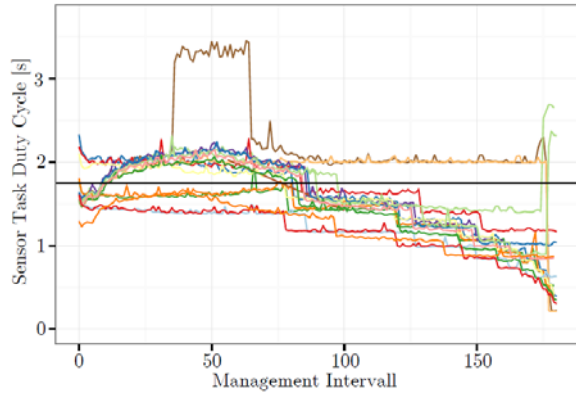
Fig. 11. Dynamically selected duty cycle of the sensing task based on available energy and consumption. Continuous black line marks fixed duty cycle of reference nodes
