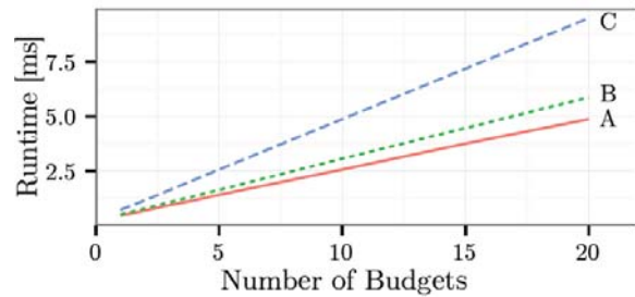
Fig. 3. Runtime of the distribution algorithm for MSP430 running at 16 MHz. (A) Based on percentage of maximal requested energy. (B) Additionally distribution of minimal requested energy. (C) Distribution of consumed/requested energy.
