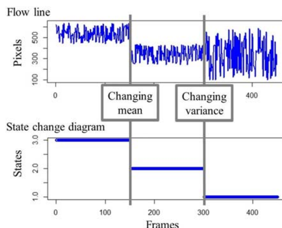
Fig. 3. State change diagram converts from flow lines.
