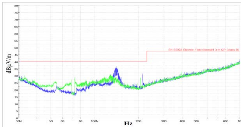
Fig. 5. Semi-anechoic chamber - the EMI of the EUT in the ON state – the antenna in the horizontal (blue line) and vertical (green line) polarization
