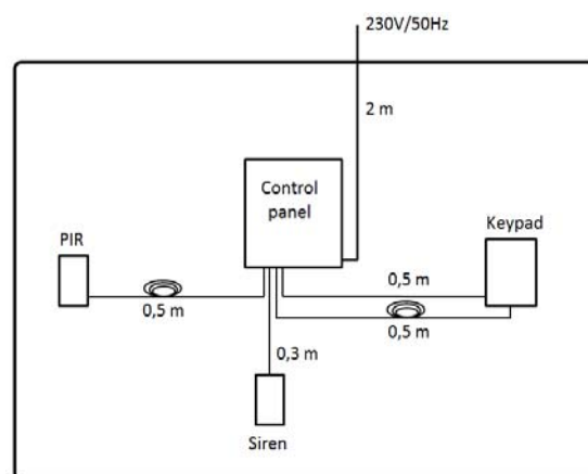
Fig. 4. The location of the components of I&HAS on the table.
