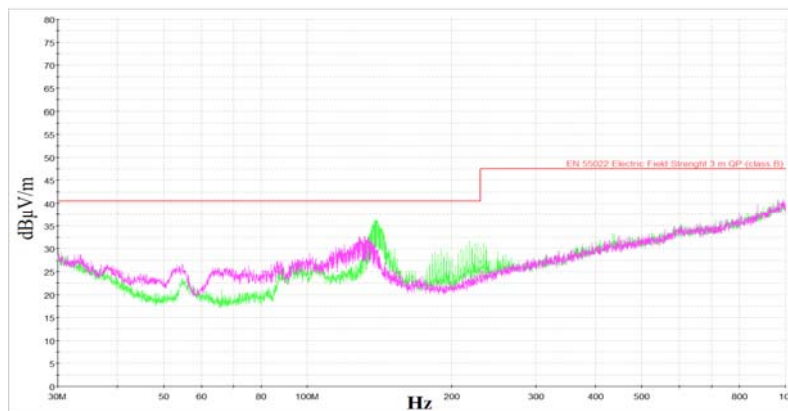
Fig. 6. Semi-anechoic chamber - the EMI of the EUT in the state of alarm – the antenna in the horizontal (green line) and vertical (violet line) polarization
