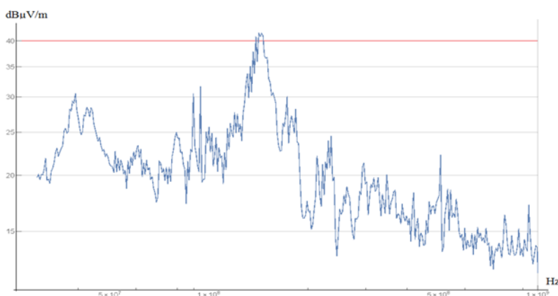
Fig. 8. GTEM cell - the EMI of the EUT in the state of alarm.
