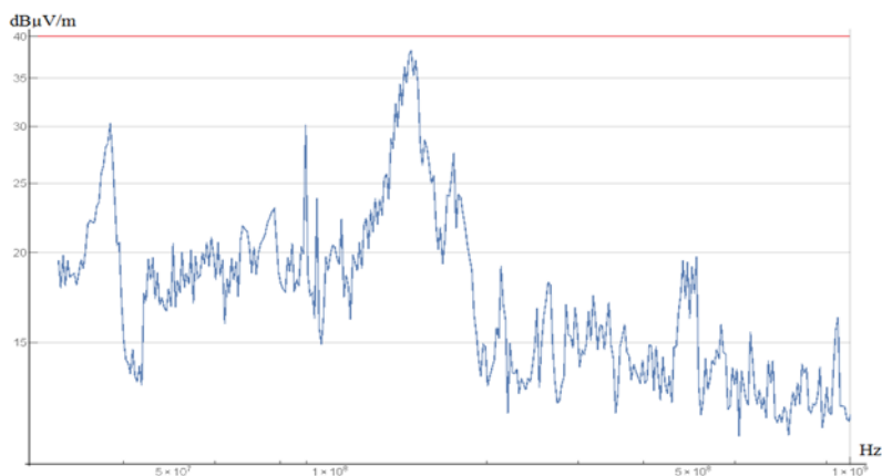
Fig. 7. GTEM cell - the EMI of the EUT in the ON state.
