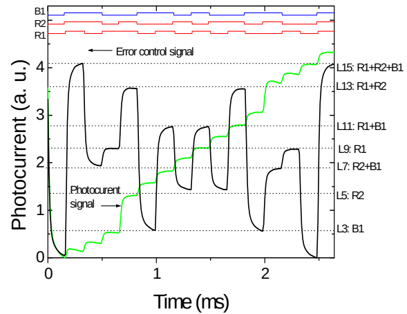
Fig. 11. Error control signal.
