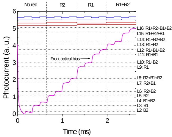
Fig. 10. Photocurrent signal measured under front optical bias using two red and two blue optical signals modulated with multiple frequencies (on the top it is displayed the waveform of the emitters modulation state).
