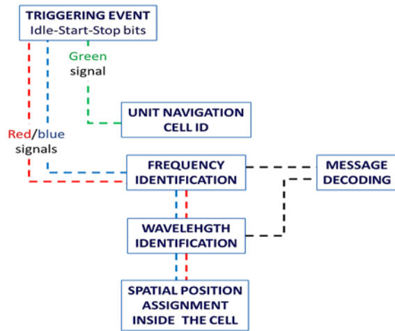
Fig. 6. Decoding tasks.
