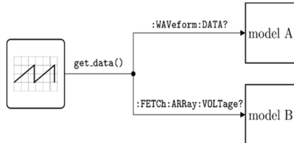
Fig. 3. Example of unique interface taking advantage of the polymorphism and encapsulation mechanisms to hide the specific SCPI commands into a single Python function.
