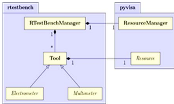
Fig. 2. R-testbench Unified Modeling Language (UML) class diagram: manager, tool interfaces mechanism, and interactions with PyVISA [5].
