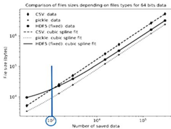
Fig. 7. Comparison of the evolution of sizes of CSV, pickle and HDF5 files with the number of data. [5]. Data are saved to files using the pandas I/O API.
