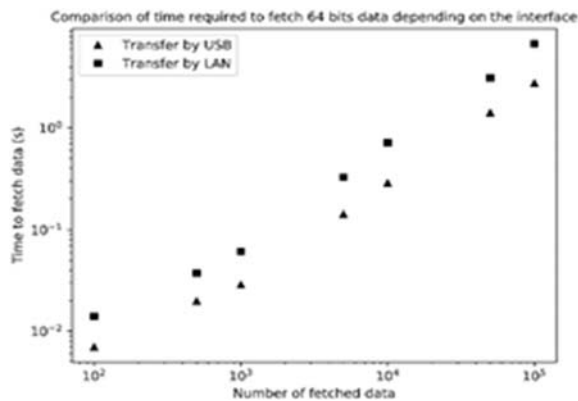
Fig. 5. Comparison of time required to fetch data from a Keysight B2985A electrometer to the computer [5]. Data are stored locally in a numpy. ndarray container.
