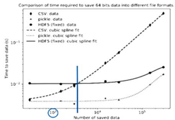
Fig. 6. Comparison of the evolution of the time required to save data into CSV, pickle and HDF5 files formats with the number of data [5]. Data are saved to files using the pandas I/O API.
