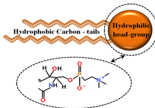
Fig. 5. Sphingomyelin: symbolic representation.
